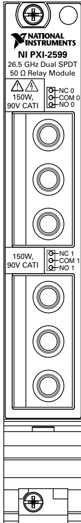
Figure 4. PXI-2599 Front Panel
