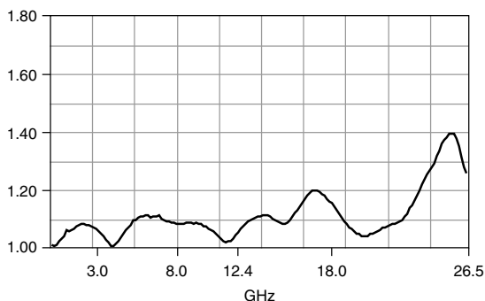
Figure 2. VSWR, Typical
