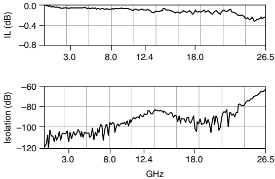
Figure 1. Insertion Loss and Isolation, Typical
